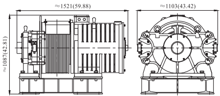
Dimensions: mm(in)
